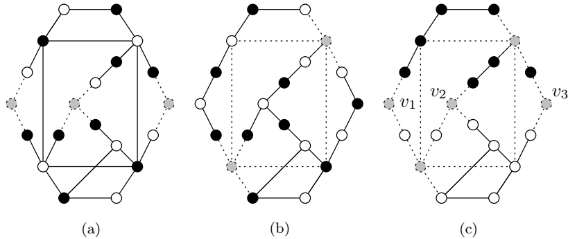
Figure 2: Comparing disjoint odd cycle covers: (a) a graph G with an odd cycle cover X (grey vertices); a two-coloring C_X of G \setminus X is marked with black and white vertices ; (b) another odd cycle cover X' of G with Properties 1–3, and a corresponding two-coloring C_{X'} ; (c) the comparison function \Phi .
